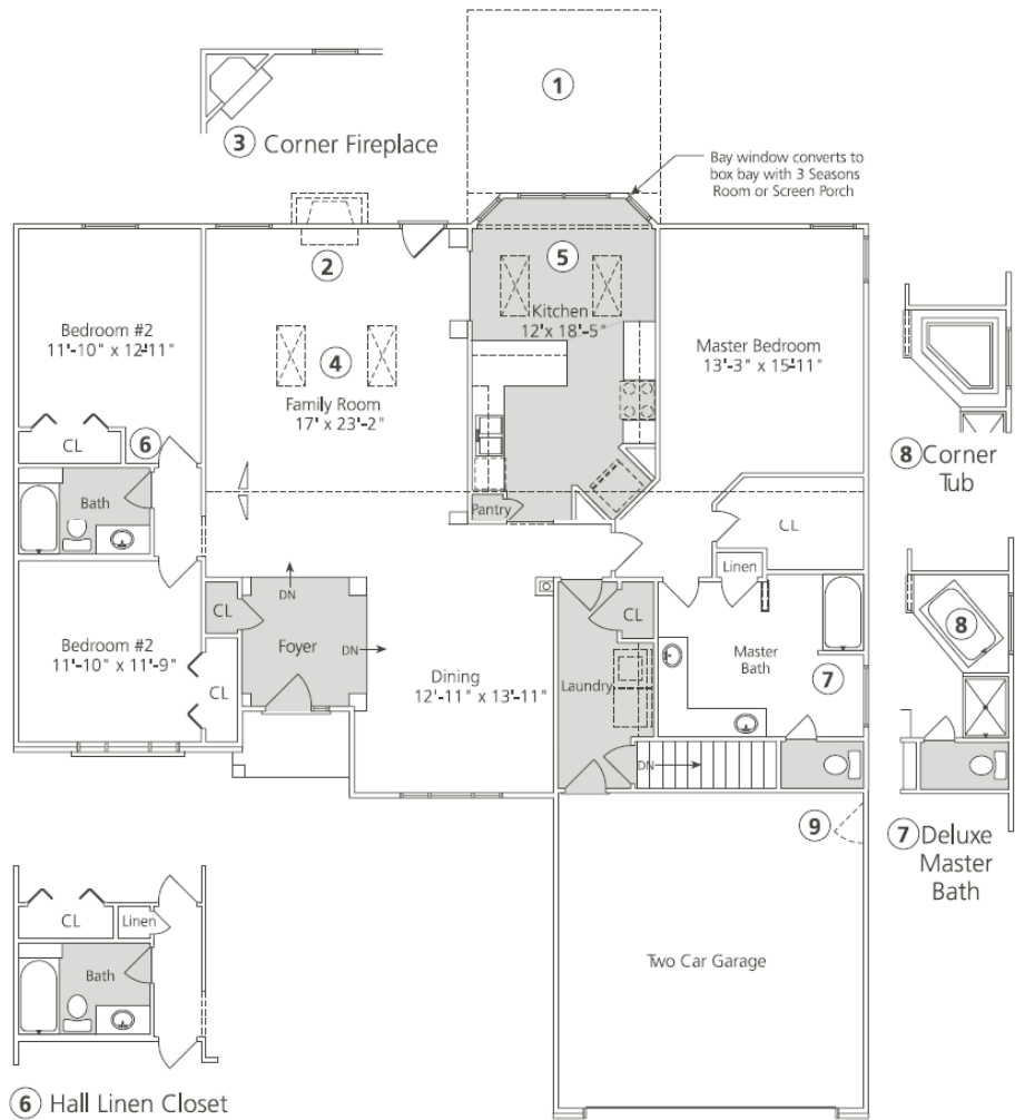
Floor Plan (Elevation "A")
